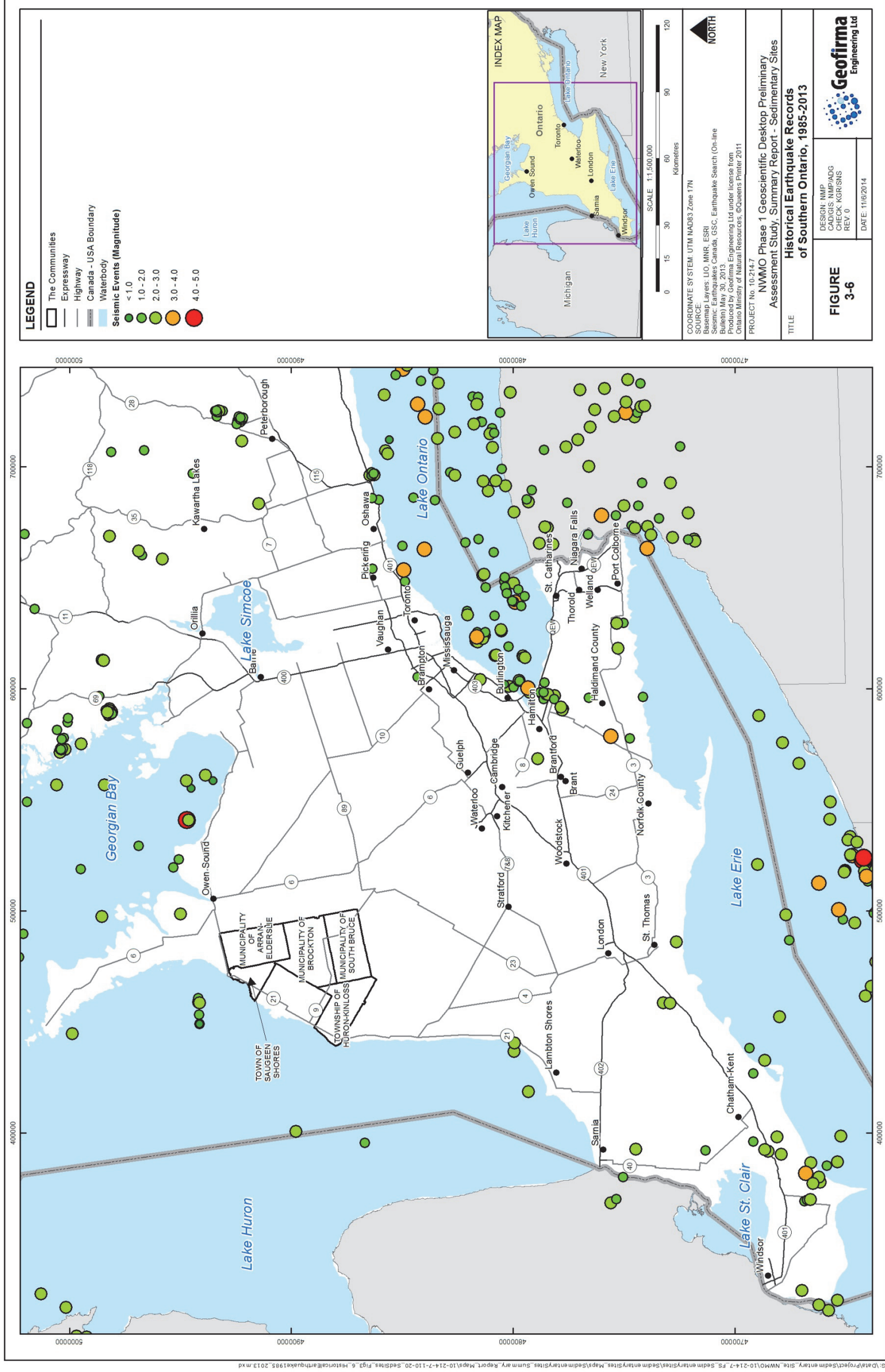
Figure 3-6: Historical Earthquake Records of Southern Ontario, 1985-2013
