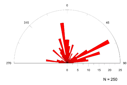
Nipigon Geophysical Brittle Lineaments - Length Weighted Frequency Rose Plot
