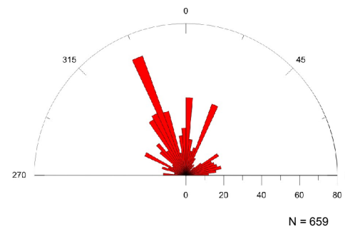
Nipigon CDED Data - Length Weighted Frequency Rose Plot
