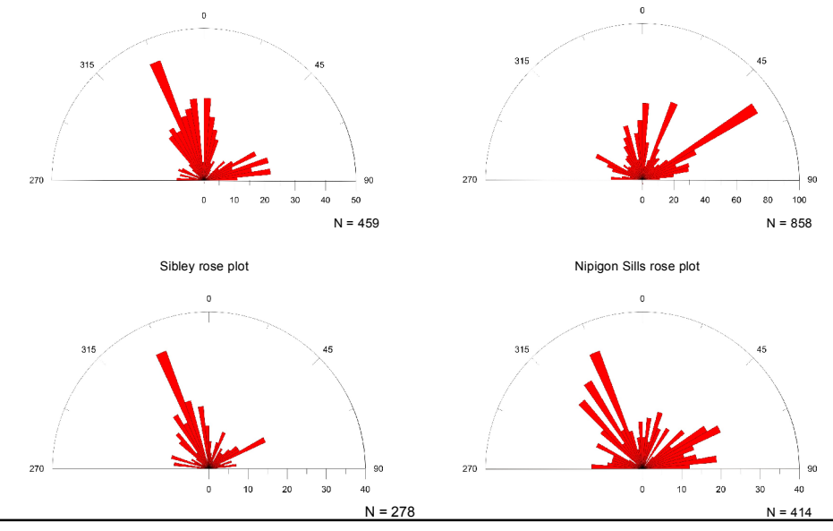
Quetico metasediments within high resolution aeromagnetic dataset Quetico metasediments outside high resolution aeromagnetic dataset
