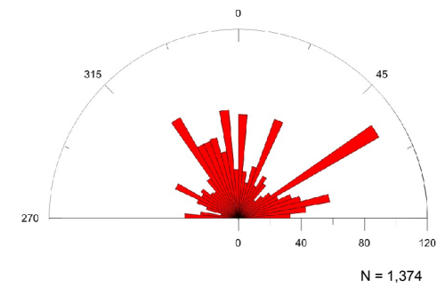
Nipigon SPOT Data - Length Weighted Frequency Rose Plot
