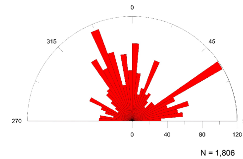
Nipigon All Data - Length Weighted Frequency Rose Plot
