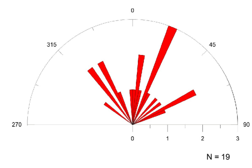
Nipigon Geophysical Dykes - Length Weighted Frequency Rose Plot
