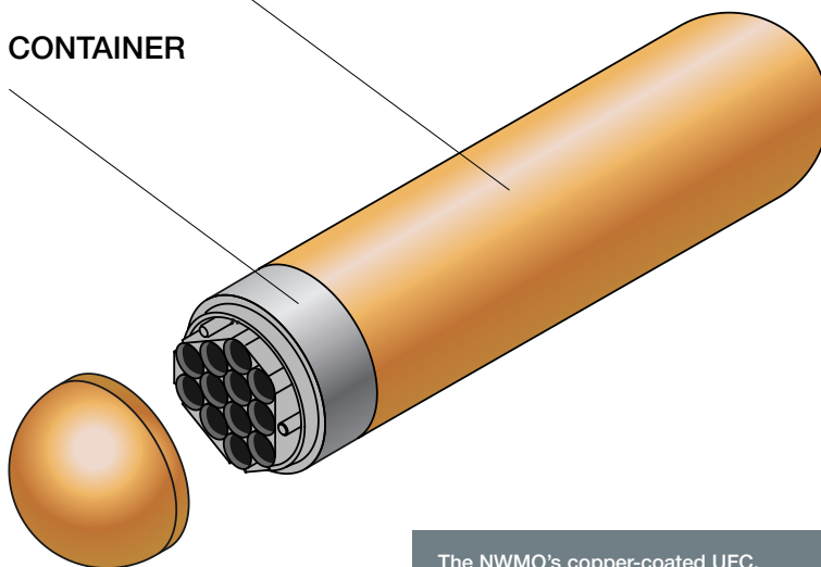
The NWMO's copper-coated UFC.
