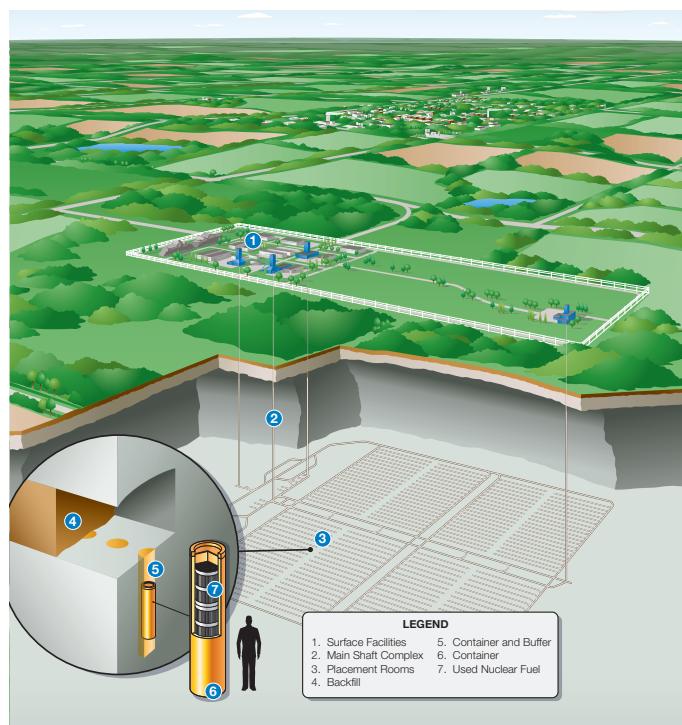
Figure 1: Monitoring and Retrieval in Adaptive Phased Management
