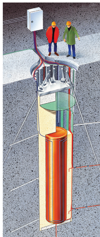
Figure 2: The Canister Retrieval Test at the Äspö Hard Rock Laboratory in Sweden
