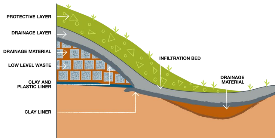
Figure 11: Engineered containment mound
