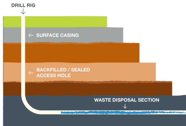
Figure 15: Deep borehole disposal
